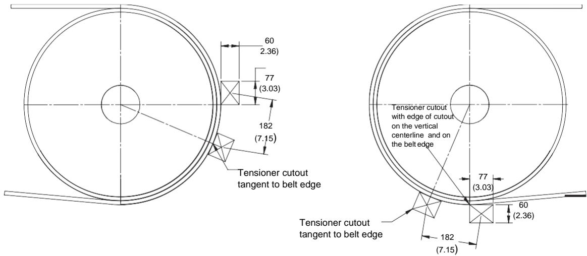
Mounting Location for CleanScrape® Medium Cleaner Requiring Tensioners on Both Sides
