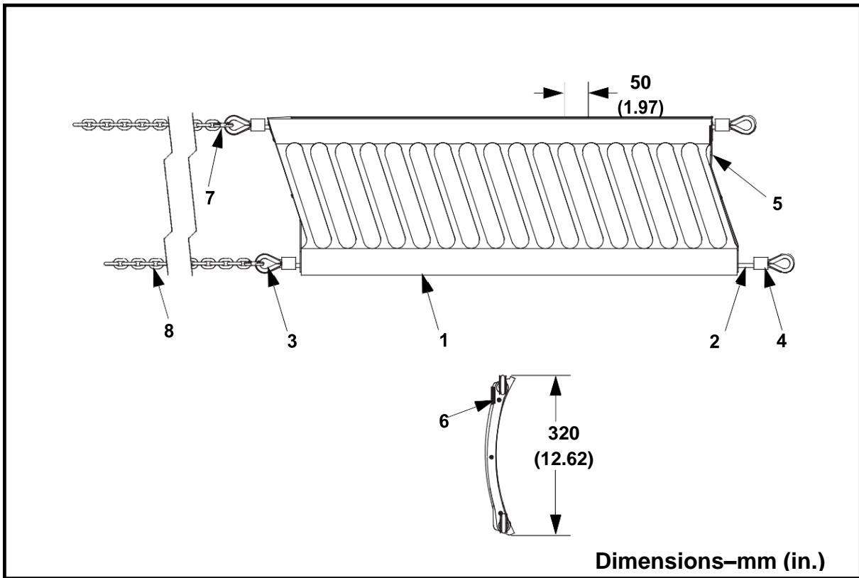
Figure 13: CleanScape® Large Cleaner, P/N C1CLRXXXXXX
