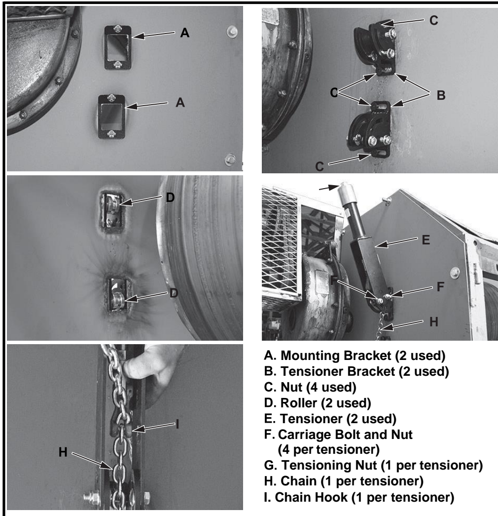
Figure 8: Installing Tensioners
