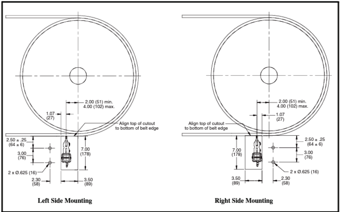
Figure 1. Mounting Locations
