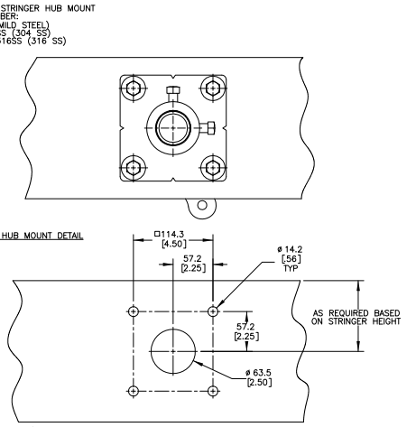
OPTIONAL HUB MOUNT STRINGER MOUNTING CUTOUT DETAIL
