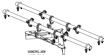
ISOMETRIC VIEW 1 PIECE FRAME FRONT AND REAR HANGER BARS THE SAME FOR BELT WIDTHS 18 AND 24 (SHOWN WITH BOLT ON URETHANE BLADE) SCALE 1:3
