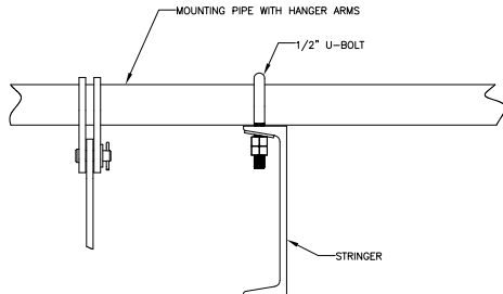
TOP OF STRINGER MOUNTING DETAIL BOTTOM OF STRINGER MOUNTING IS SIMILAR DRILL HOLES IN STRINGER AS SHOWN CLAMP MOUNTING PIPE TO STRINGER WITH U-BOLTS SCALE 5:16
