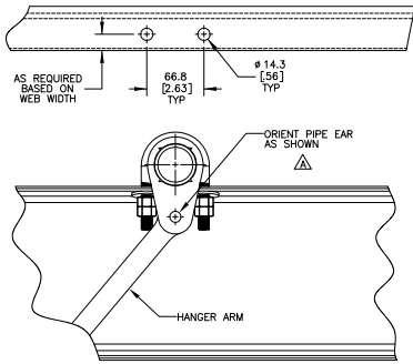
TOP OF STRINGER MOUNTING DETAIL BOTTOM OF STRINGER MOUNTING IS SIMILAR DRILL HOLES IN STRINGER AS SHOWN CLAMP MOUNTING PIPE TO STRINGER WITH U-BOLTS SCALE 5:16
