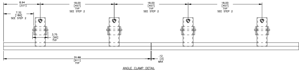
ANGLE CLAMP DETAIL
