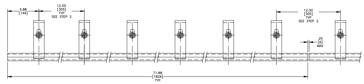
ANGLE CLAMP DETAIL
