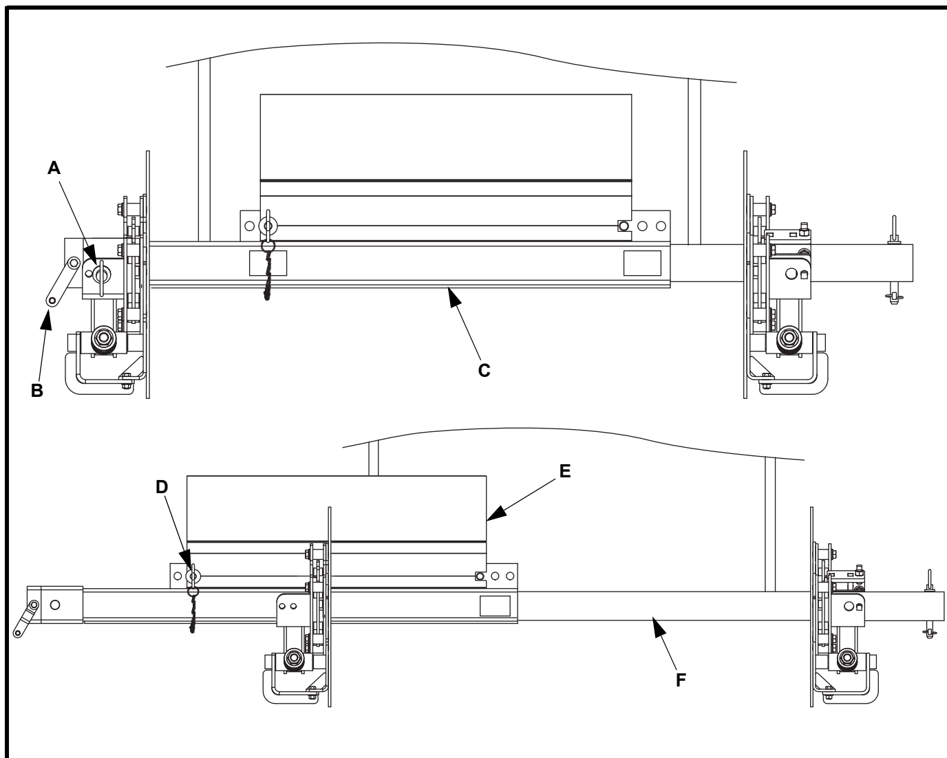
Figure 8. Blade Replacement
