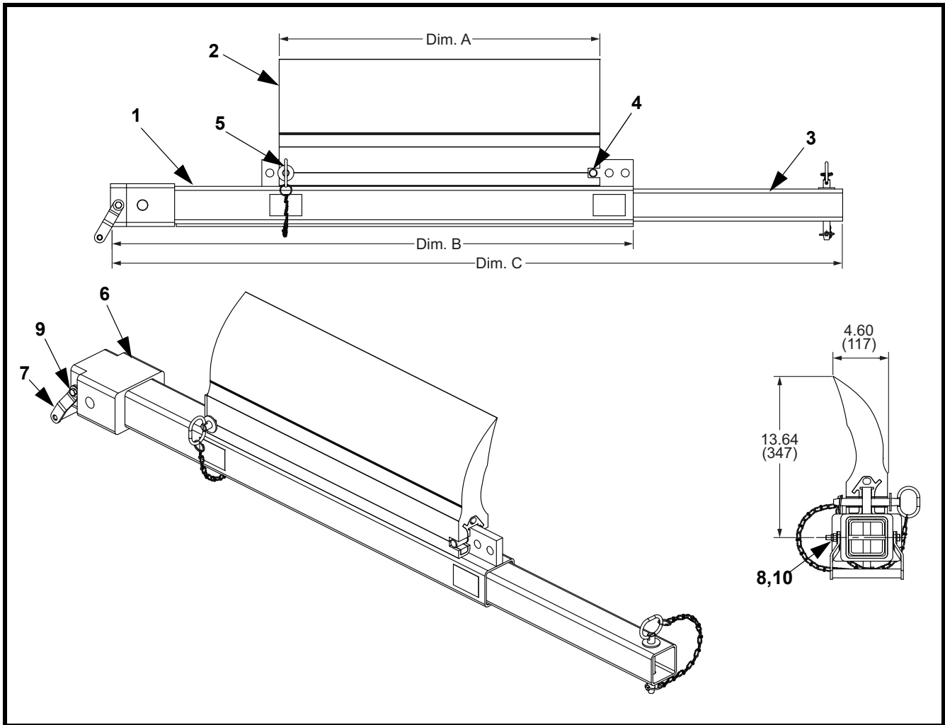
Figure 9. Martin® QC1™ Cleaner XHD STS™ Assembly, P/N STSXHDQC-XXXXXXXXX
