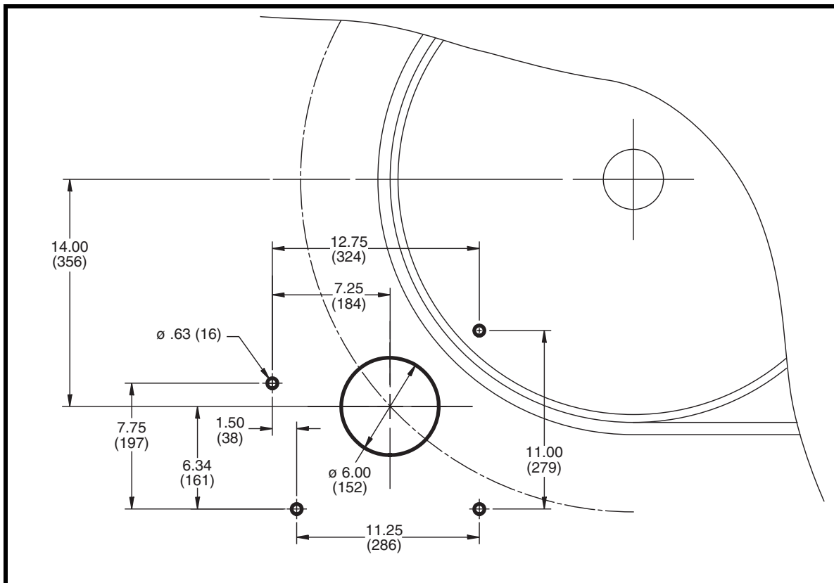
Figure 4. Far Side Chute Cutout
