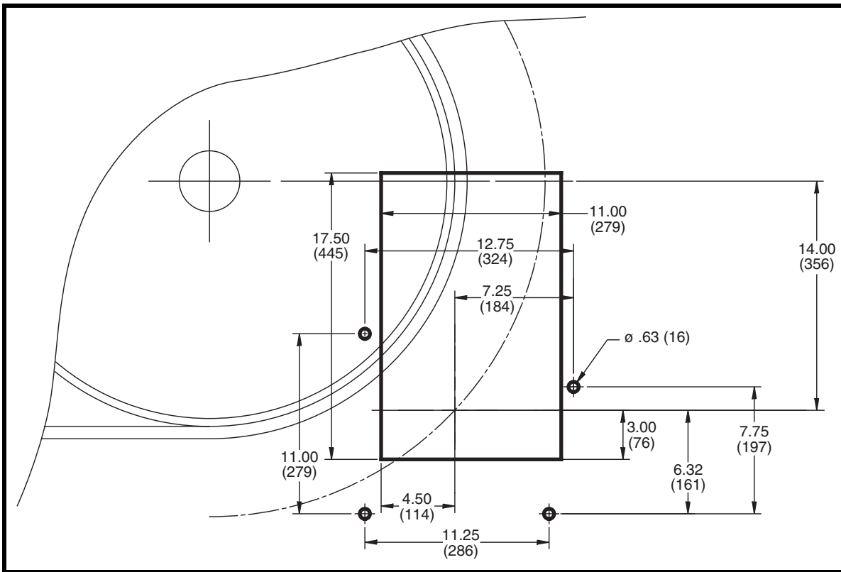
Figure 3. Operator Side Chute Cutout
