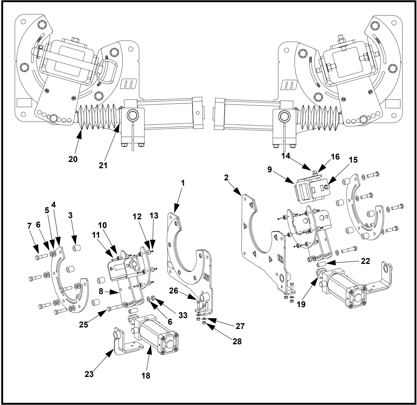
Figure 11. Martin® Air Cylinder Tensioner XHD STS™, P/N 39100-XHDASQ
