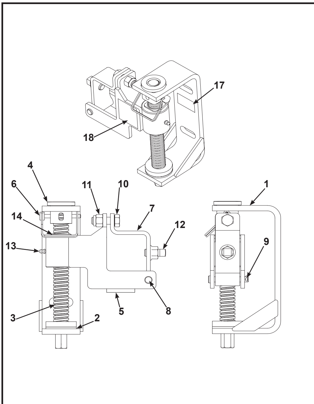
Figure 1. Martin® SQC2S™ Square Mainframe Tensioner Assembly, P/N 38664
