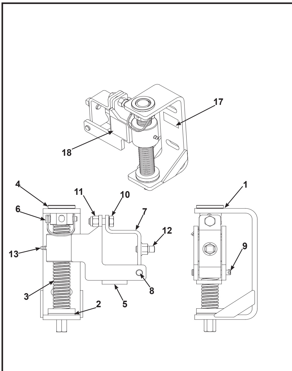
Figure 2. Martin® SQC2S™ Square Mainframe Tensioner HD Assembly, P/N 38664-HD
