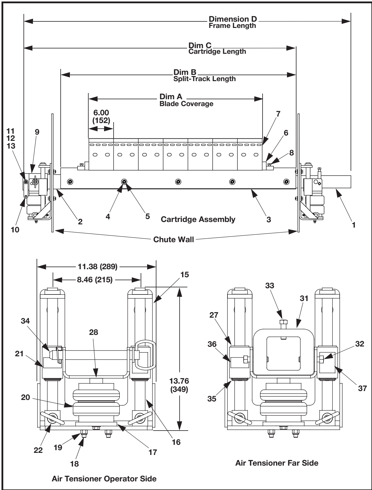
Figure 4. Martin® DT2H Reversing Cleaner XHD Assembly, P/N DT2H-XXXXXXXXXA with Air Tensioner, P/N 37806-A
