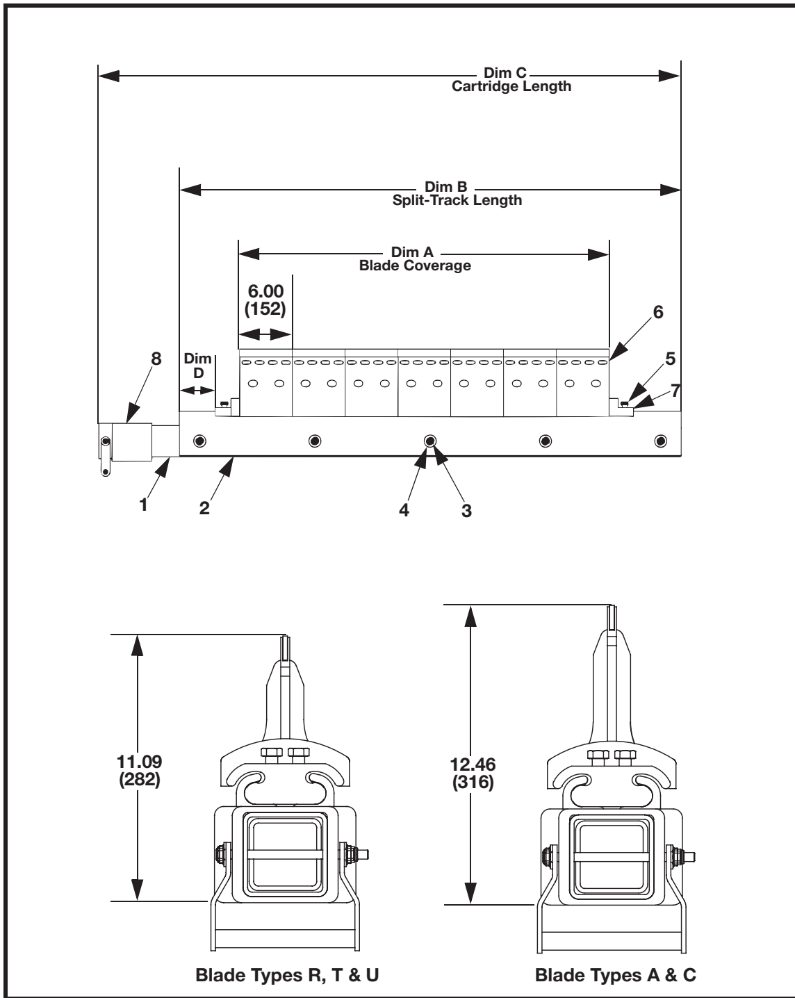
Figure 6. Martin® DT2H Reversing Cleaner XHD Cartridge, P/N DT2HC-XXXXXXXXXX
