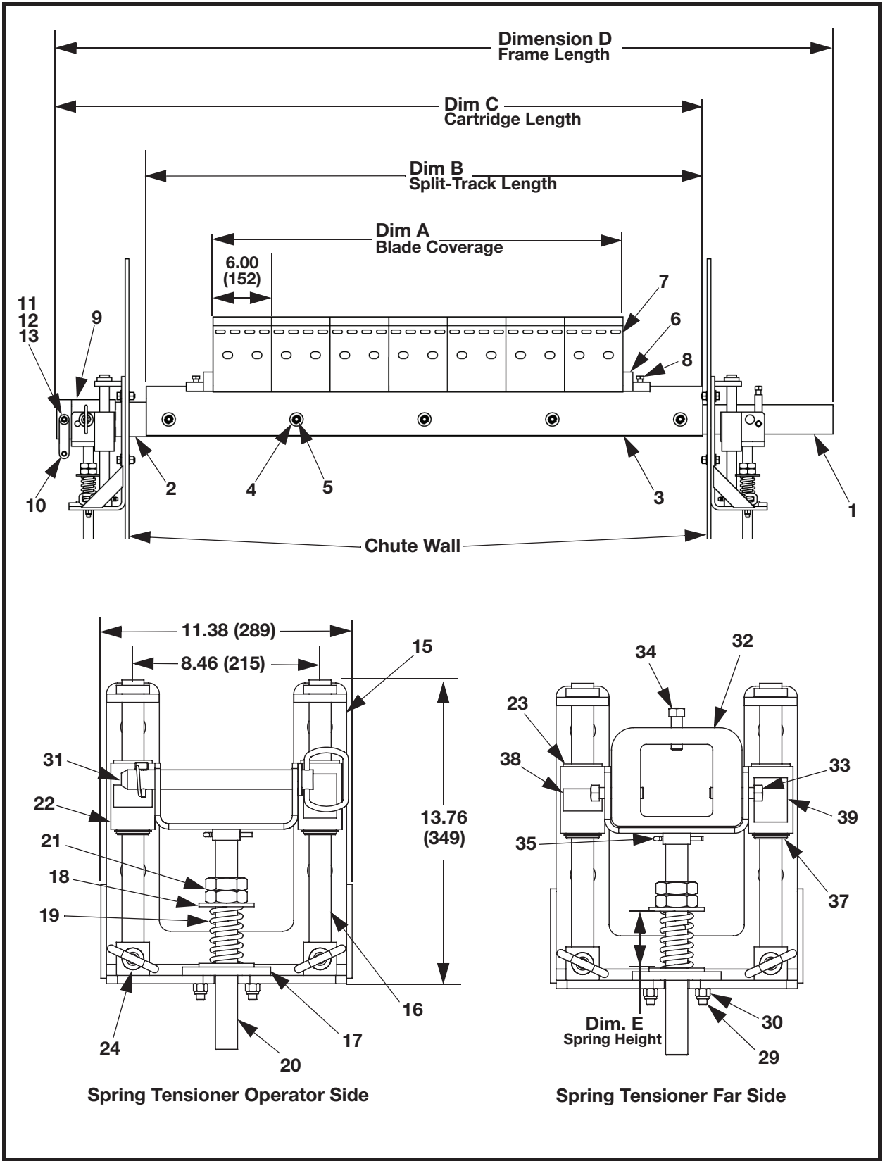
Figure 5. Martin® DT2H Reversing Cleaner XHD Assembly, P/N DT2H-XXXXXXXXXS with Spring Tensioner, P/N 37806
