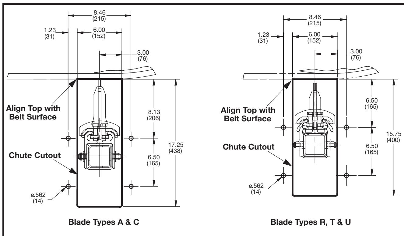
Figure 2. Chute Cutouts
