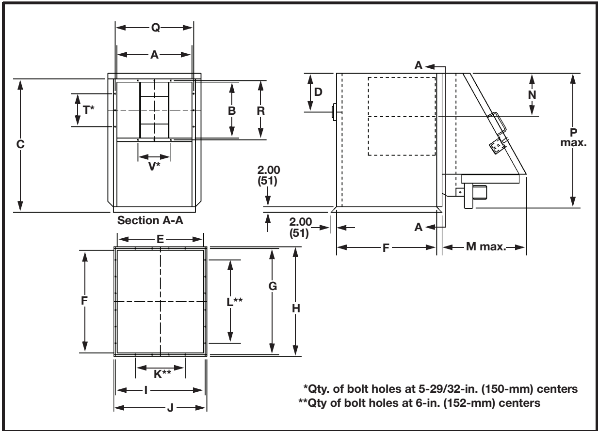
Figure 2. Dimensions for Horizontal Upstands† in. (mm) (Part 1 of 2)
