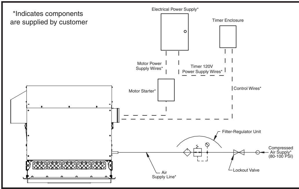
Figure 4. Electrical and Plumbing Detail
