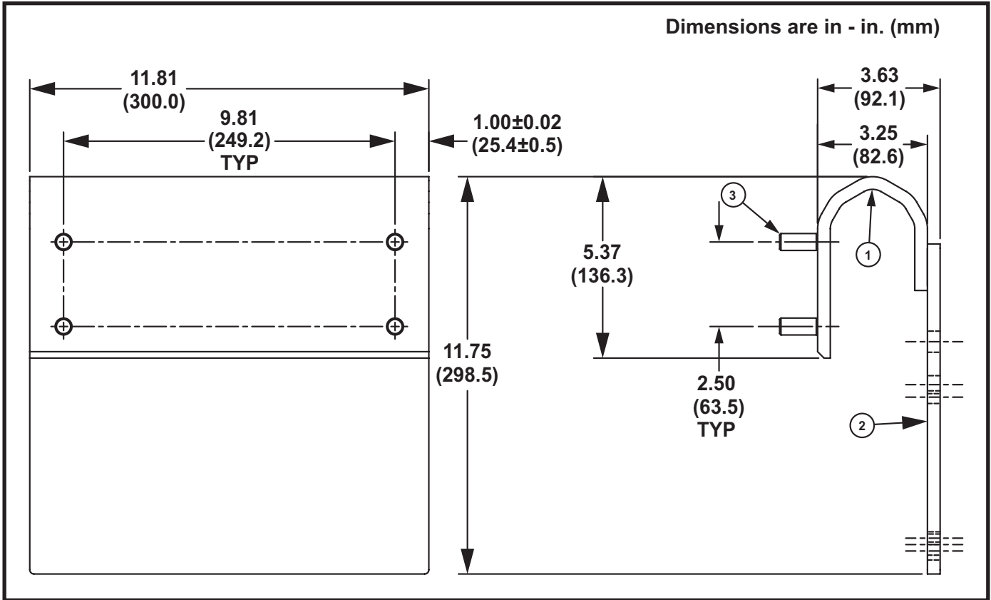
Figure 6. Dribble Chute Bracket, P/N 31496 (For Frame Sizes 00, 01, 10 Vibrators)
