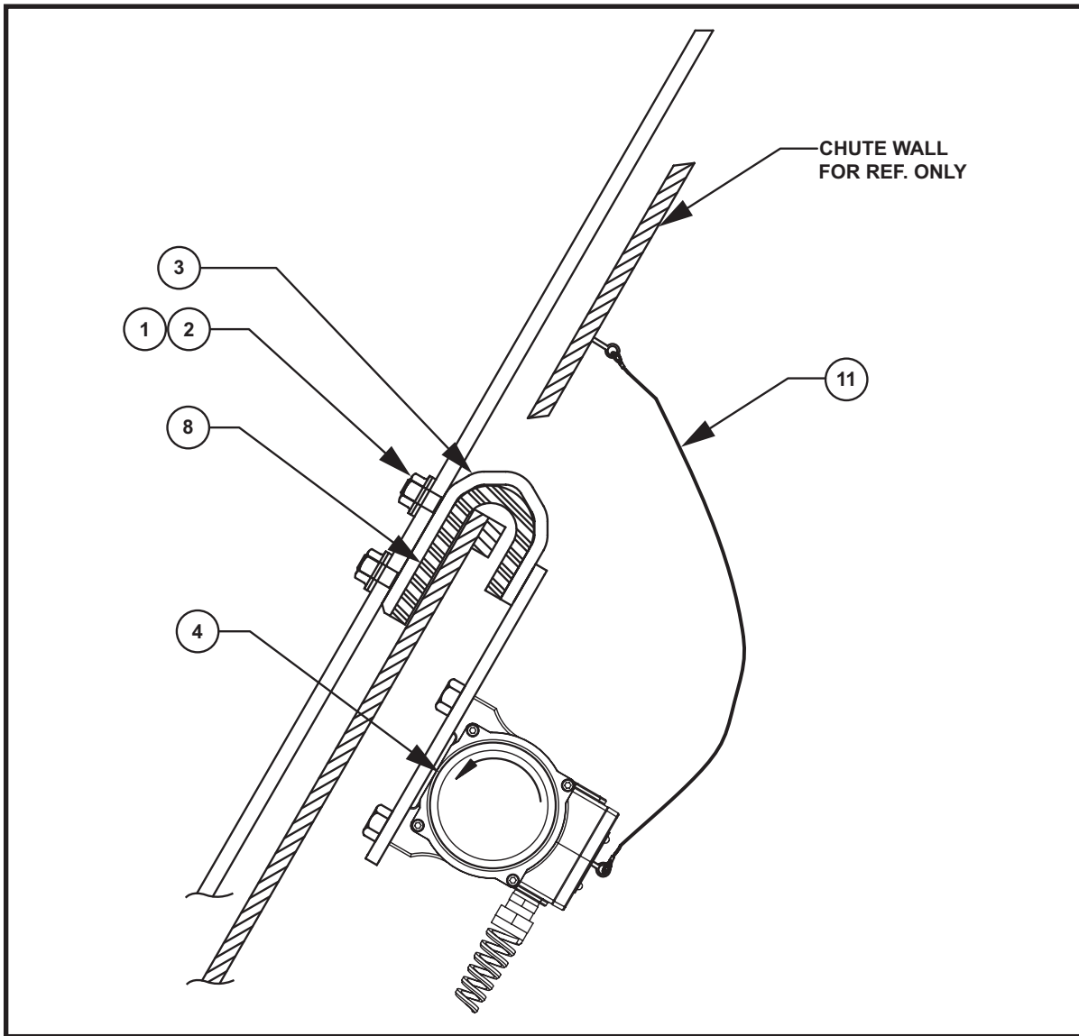
Figure 4. Martin® Vibrating Dribble Chute Assembly, P/N 31546
