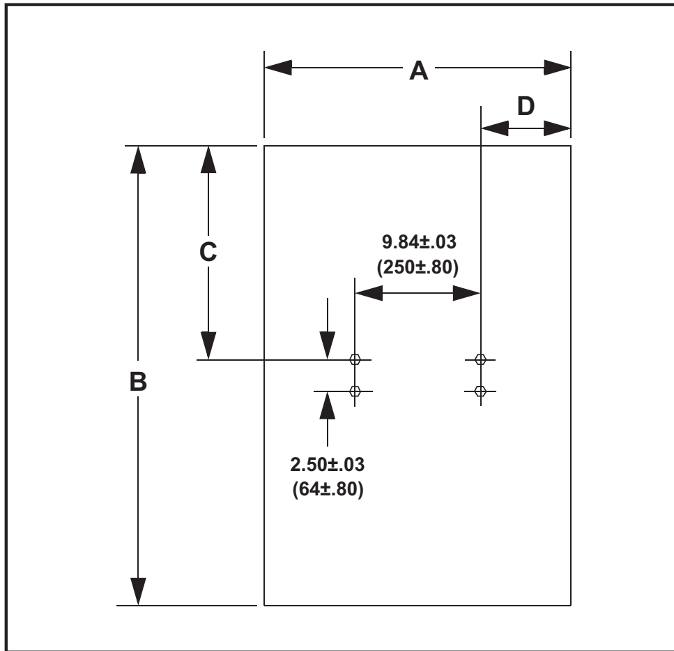
Figure 5. Dribble Sheet, P/N 31494-XXXXXX*
