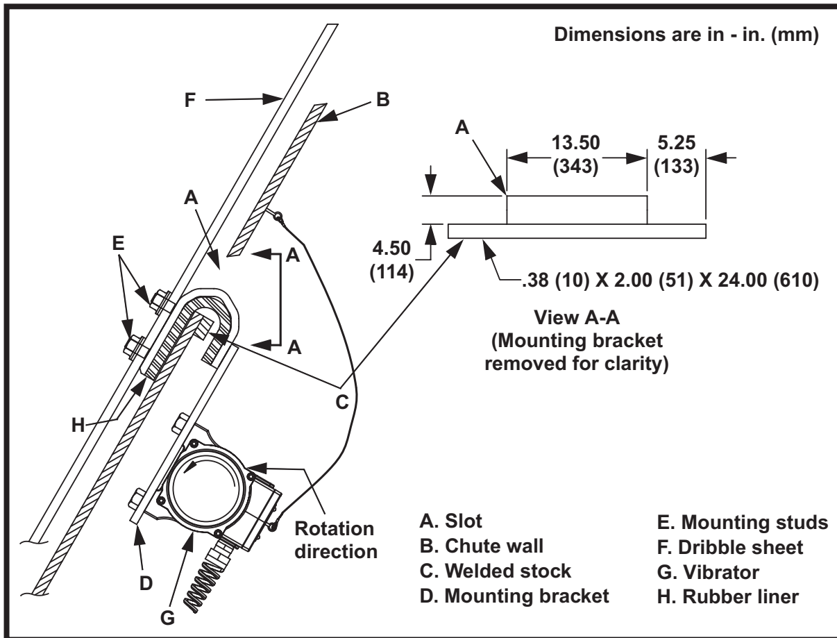
Figure 2. Dimensions for Slot and Welded Stock
