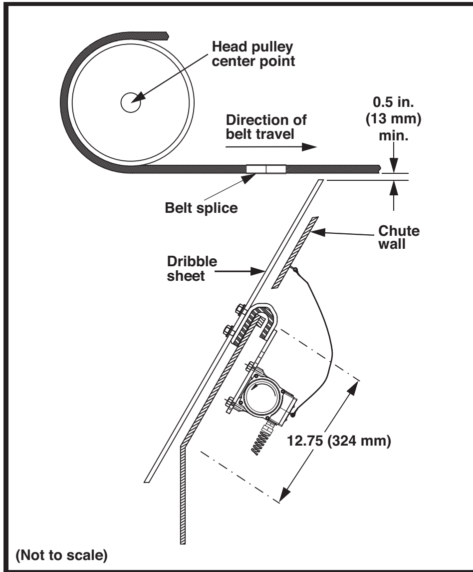
Figure 1. Minimum Clearance for Vibrating Dribble Chute Installation
