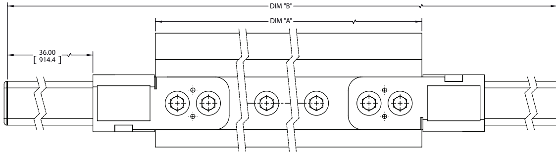
Martin® UBX Secondary Cleaner Assembly With Metal Blade Shown Above. P/N: UBMSXXSXXXX
