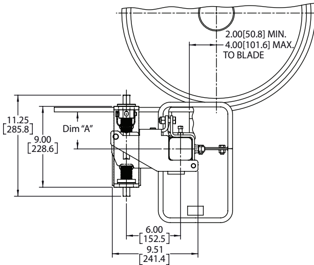
Detail With Tensioner Mounted On Left Side
