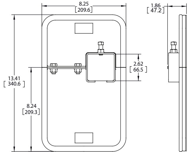
Martin® UBX Secondary Cleaner Cover Door Detail
