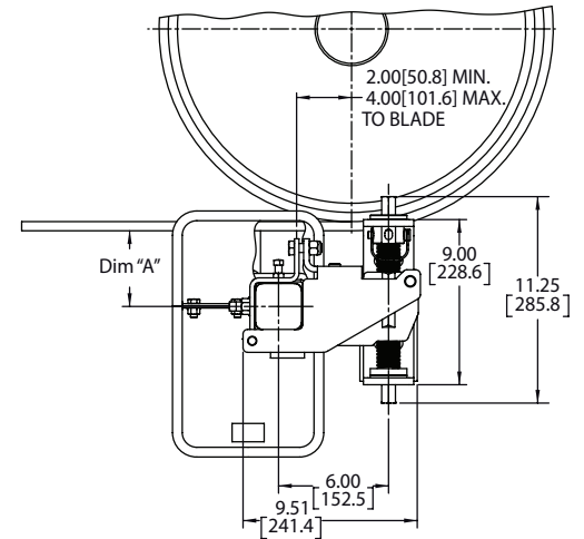
Detail With Tensioner Mounted On Right Side
