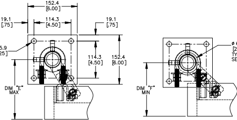
MAINFRAME LOCATION DETAIL SCALE 1:4
