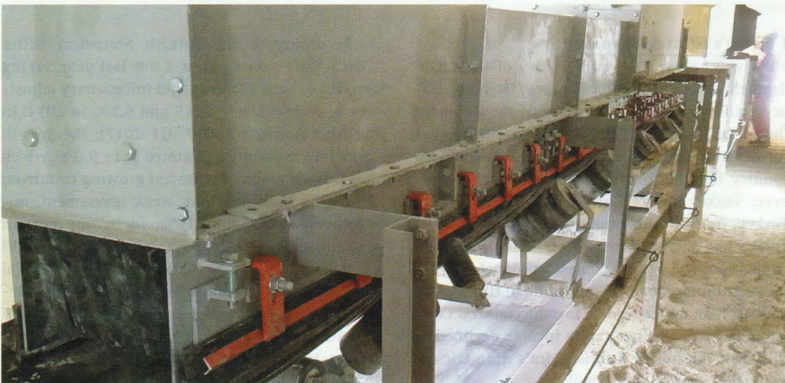
4 The EVO External Wear Liner helps prevent damage to the chute wall
