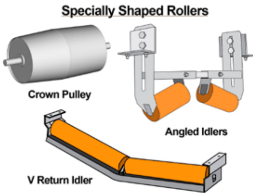
1 Different component designs for improving belt alignment
