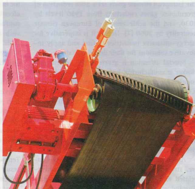
3 The track-mounted Martin Slider Cradle can be serviced quickly and safely, with no reach-in maintenance
