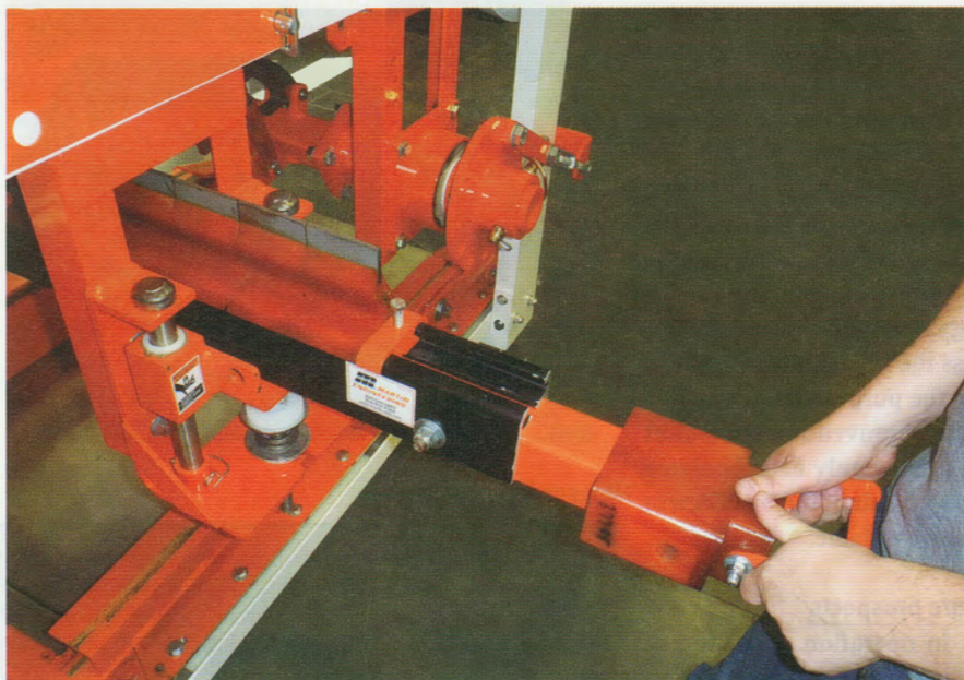
2 This Martin SQC2S™ STS secondary cleaner allows for safe external maintenance by a single worker
