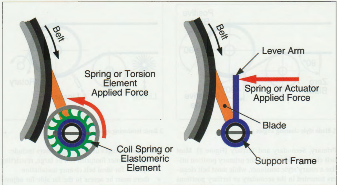
5 Rotary tensioner types
