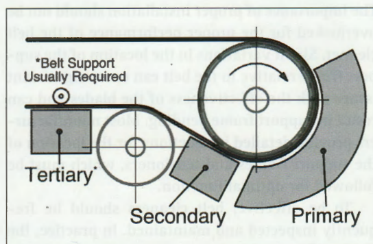
3 CEMA-defined cleaning positions
