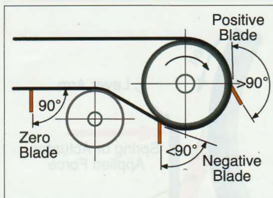
1 Blade style cleaning angles
