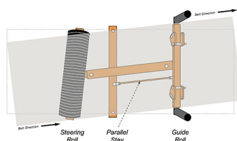
The pivoting ribbed roller design grabs the belt and uses the opposing force to shift it back into alignment.
