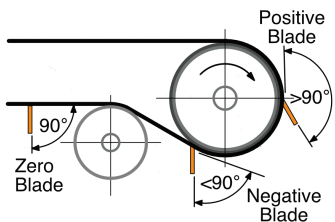
Figure 1 - Blade style cleaning angles
