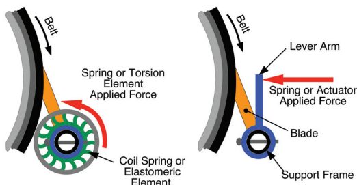
Figure 5 - Rotary tensioner types
