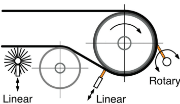
Figure 2 - Basic tensioning approaches
