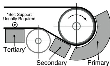
Figure 3 - CEMA-defined cleaning positions
