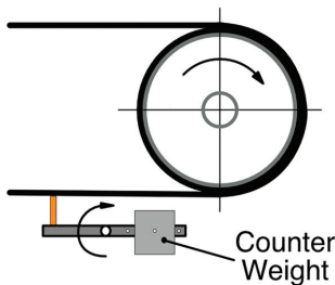
Figure 4 - Typical counterweight tensioner
