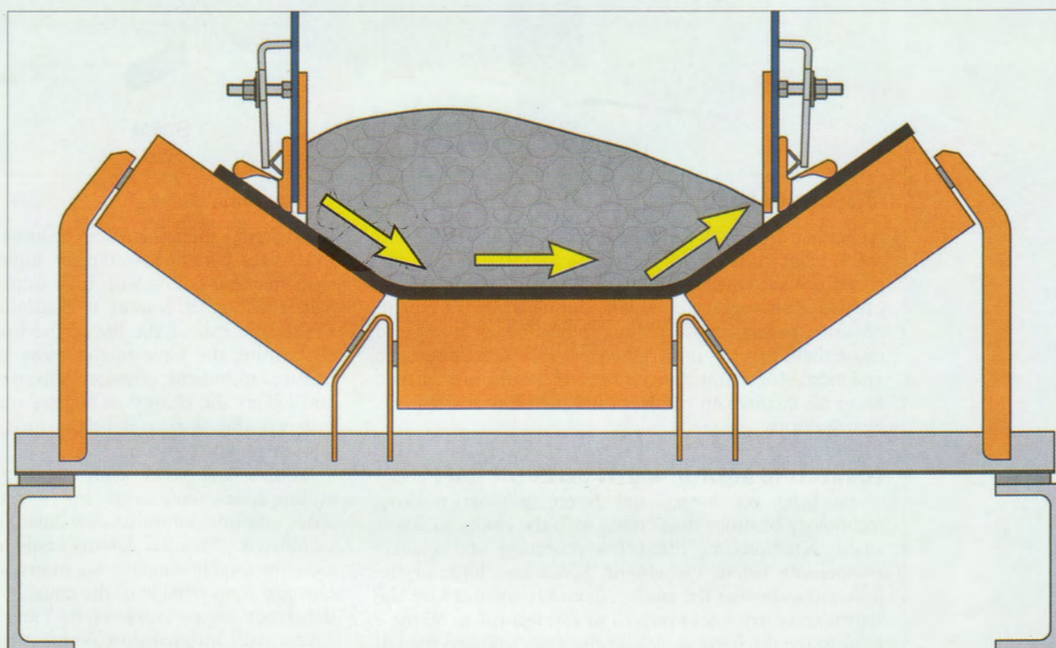
When a conveyor isn't centre-loaded, the cargo pushes the belt toward the more lightly-loaded side.
