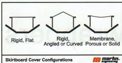
Figure 4: Angled or semi-circular covers are often used when rain protection or buildup of fugitive materials is a concern.
