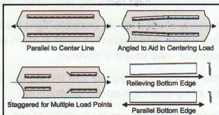
Figure 5: Reversing belts must use skirtboards parallel to the belt.
