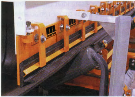
The raised skirtboard allows room for the external wearliner to perform its function and be changed easily from outside the system.
