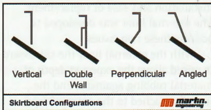
Figure 1: The most common configuration is the vertical skirtboard.
