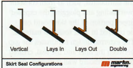
Figure 2: A Vertical seal with a rubber or elastomeric material is the most common sealing system.
