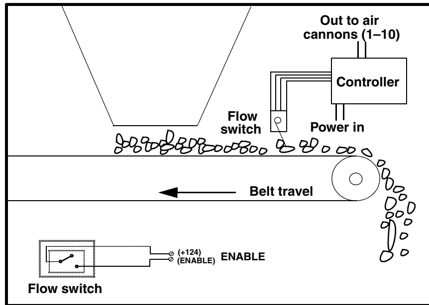
Figure 1. Flow switch inputs open, controller disabled
