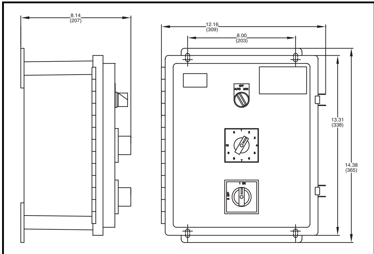
Figure 11. Air Cannon Controller Dimensions
