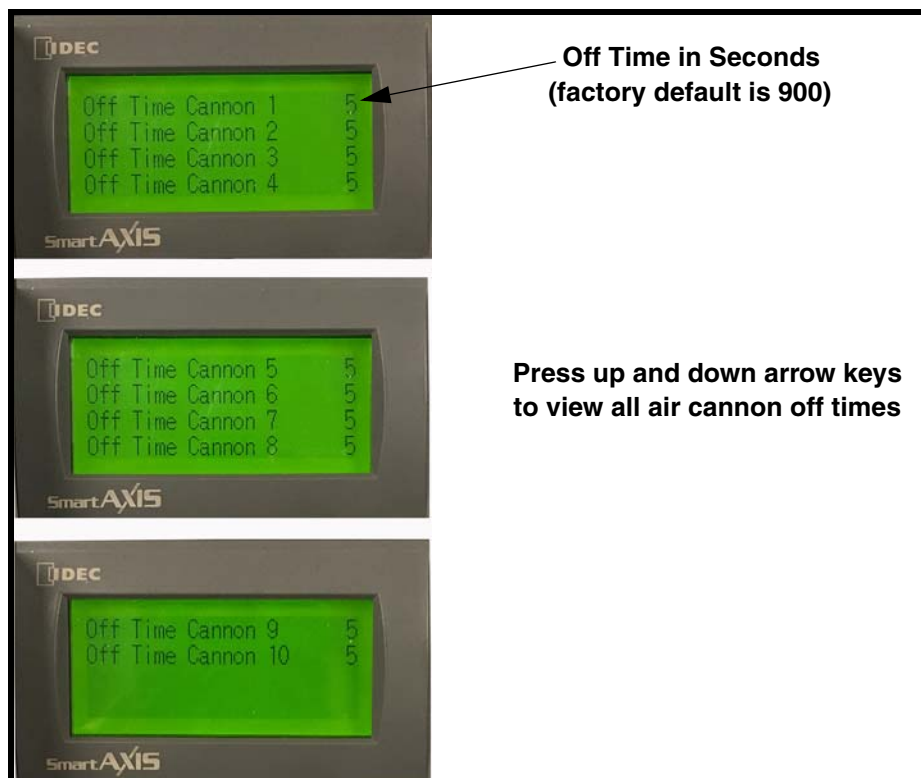
Figure 8. Air Cannon Off Time Screens
