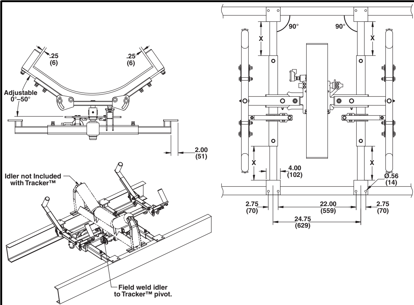
Figure 3. Mounting Dimensions–Martin® Tracker™ Reversing (Upper Unit)
