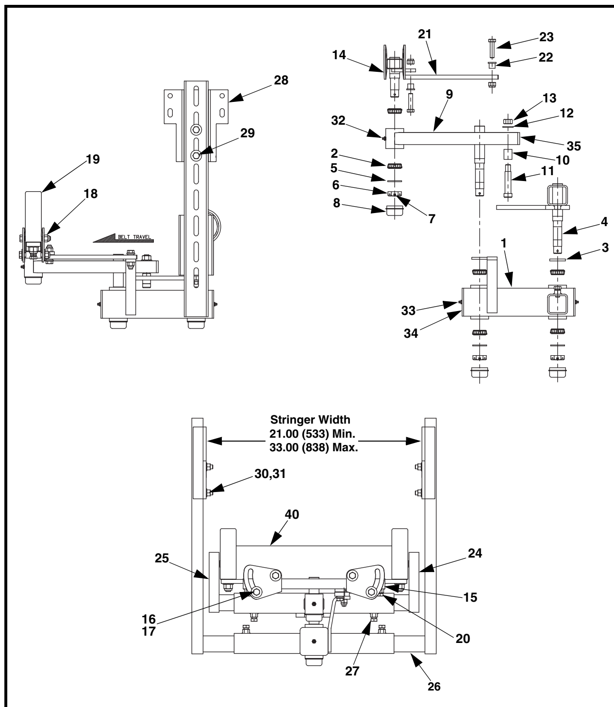
Figure 5. Martin® Tracker™, P/N TKR-18LSXX* (Sheet 1 of 2)
