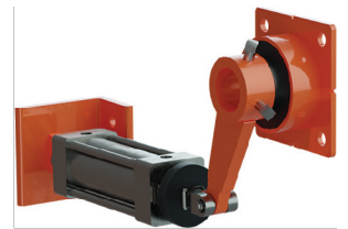
Air Cylinder Tensioner
