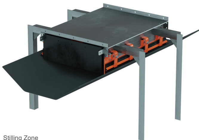
Stilling Zone
