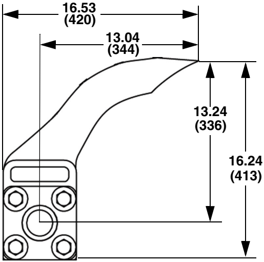
SHD-600 Blade Profile
