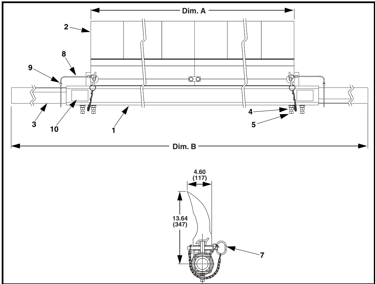
Figure 5. Martin® QC1™ Cleaner XHD Dual Blade Assembly, P/N 35899DXXXXXXXXXX*
