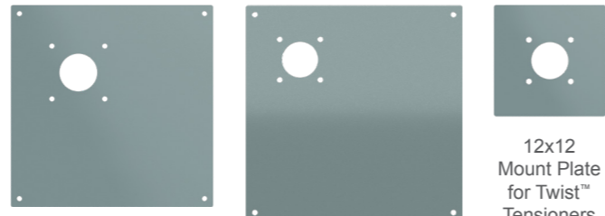
Mount Plate for XHD Spring Tensioners P/N: 39456-PXH02 Mount Plate for Twist™ Tensioners P/N: 39456-P2 12x12 Mount Plate for Twist™ Tensioners P/N: 39487-P
