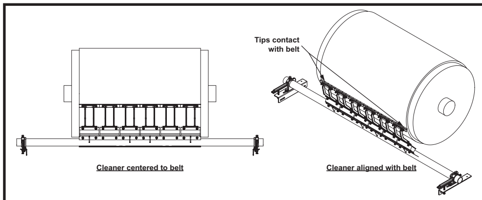
Figure 8. Martin® H1 Primary Belt Cleaner HD Tip Contact
