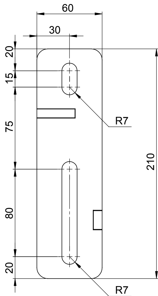
BRACKET MOUNTING DETAIL
