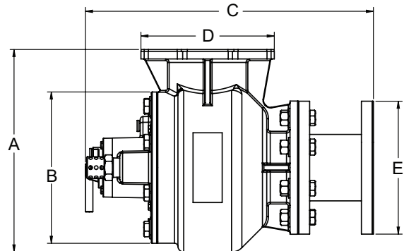
P/N 39558-H SA Positive Pressure Firing
