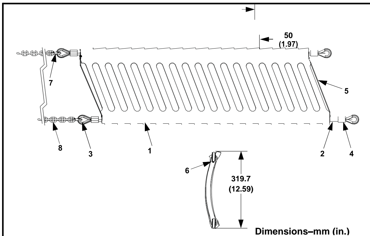
Figure 14: CleanScape® HD Cleaner, P/N C1CHXRXXXXXX
