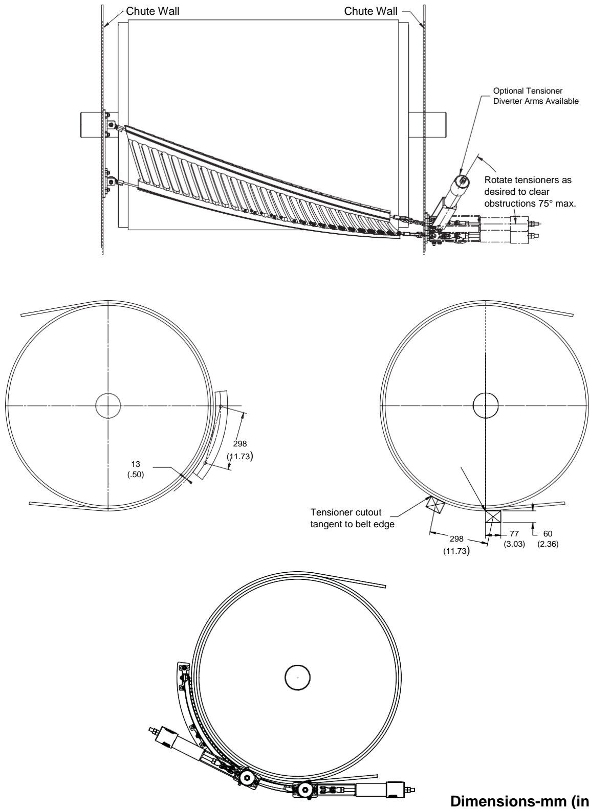
Bottom Side Tensioner Mounting for CleanScape® Large and HD Cleaners
