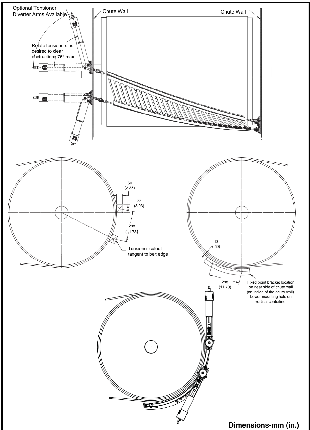
Preferred Mounting Location for CleanScape® Large and HD Cleaners
