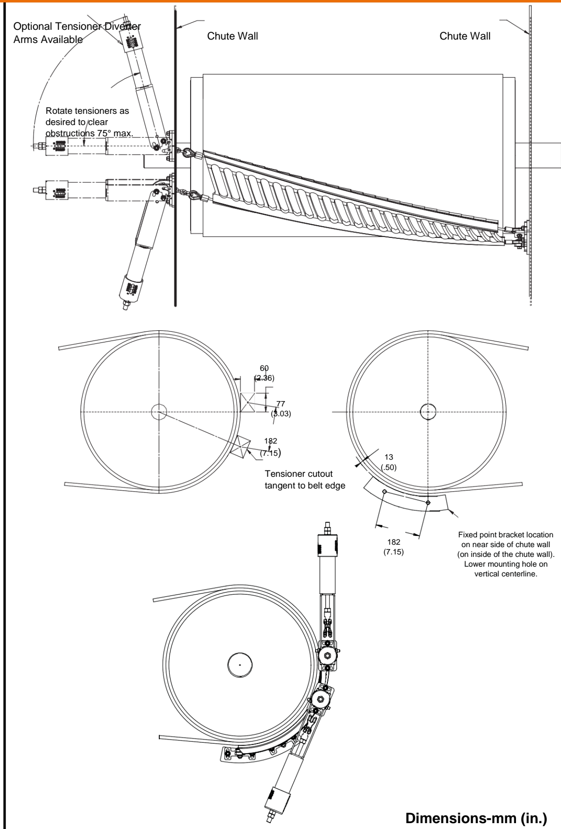
Preferred Mounting Location for CleanScape® Medium Cleaner
