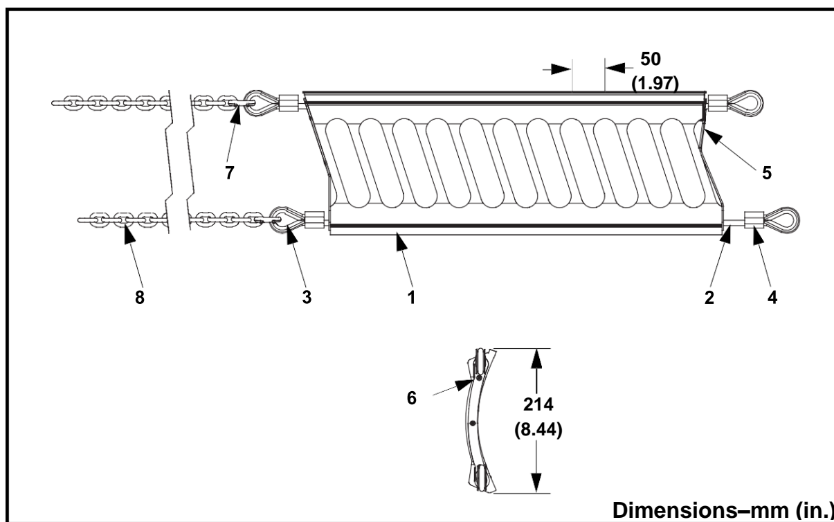
Figure 12: CleanScape® Medium Cleaner, P/N C1CMXRXXXXXX
