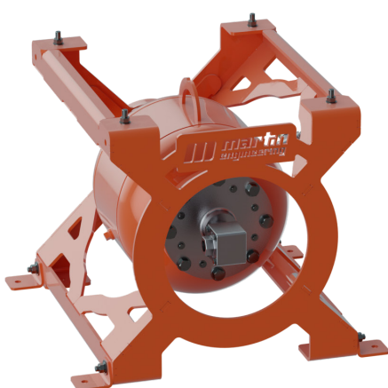
AIR CANNON X-STAND AND TYPHOON AIR CANNON
