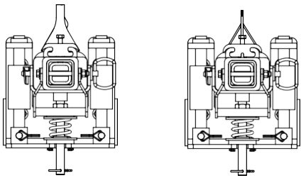
Spring Tensioners
