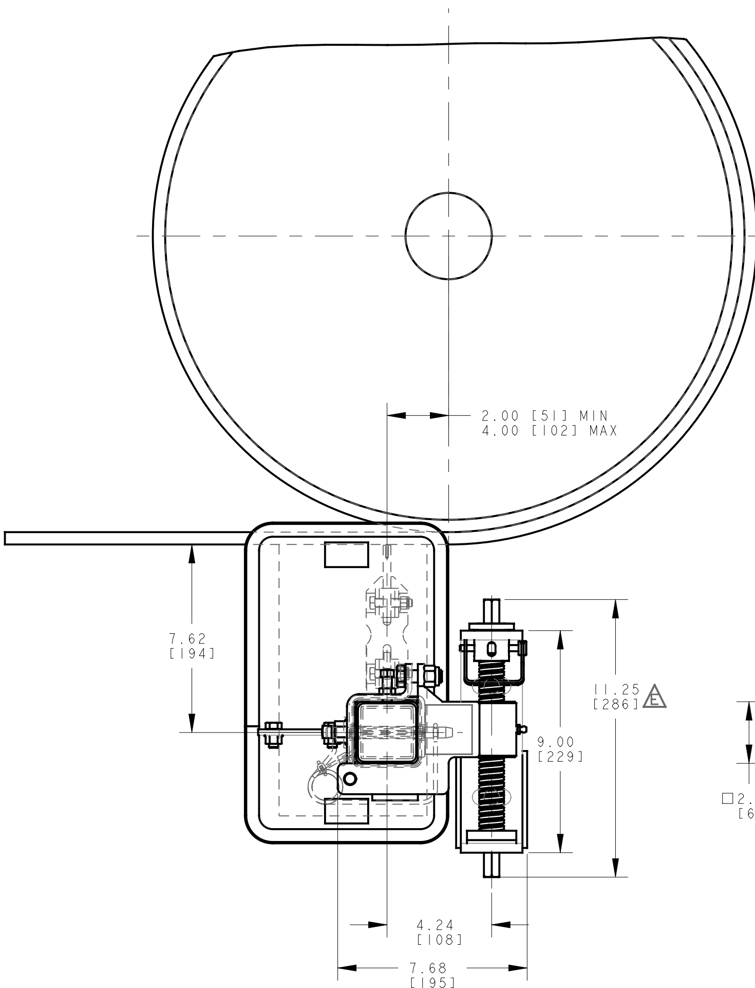
DETAIL WITH TENSIONER MOUNTED ON RIGHT SIDE
