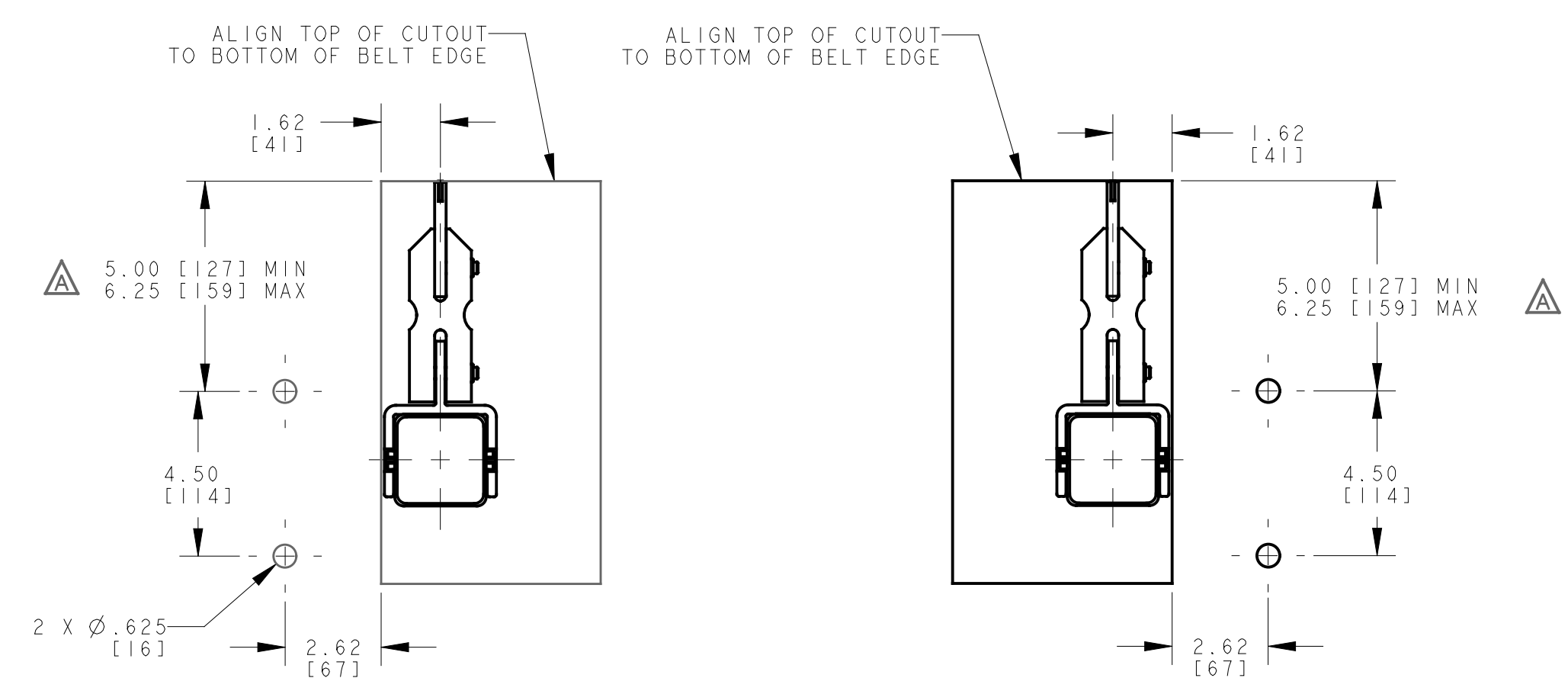
CHUTE CUTOUT DETAIL WITH TENSIONER MOUNTED ON THE LEFT SIDE SEE NOTE 10
