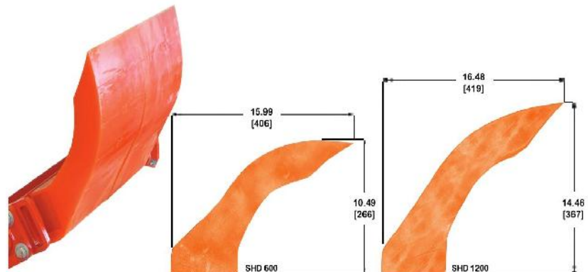
Martin® SHD Cleaner Replacement Blade
