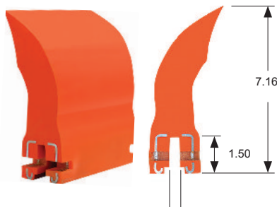
Martin® XHD Cleaner Replacement Blade
