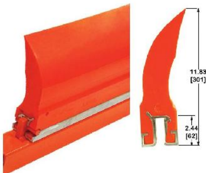
Martin® XHD Cleaner Replacement Blade
