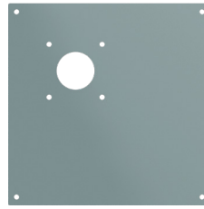
Mount Plate for XHD Spring Tensioners P/N: 39456-PXH02
