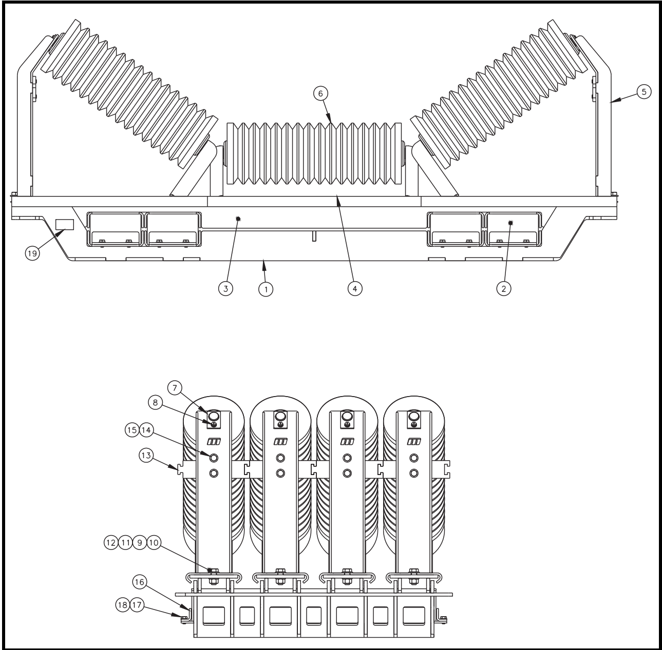
Figure 2. EVO ® High Speed Impact Cradle, P/N HSRCXXP-XXXXX
