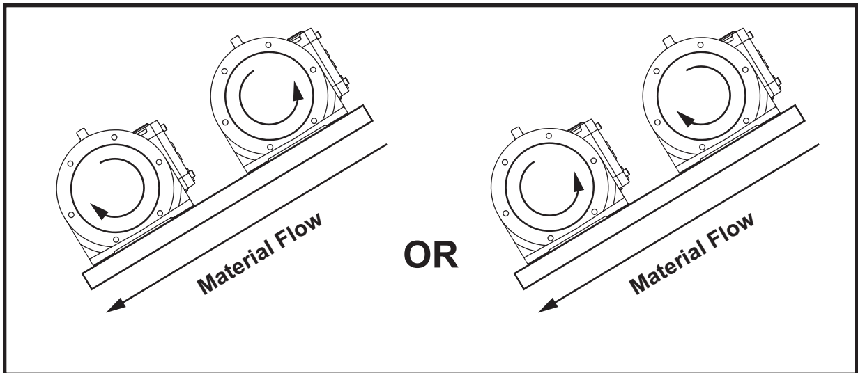
Figure 8. Two-Vibrator Screen
