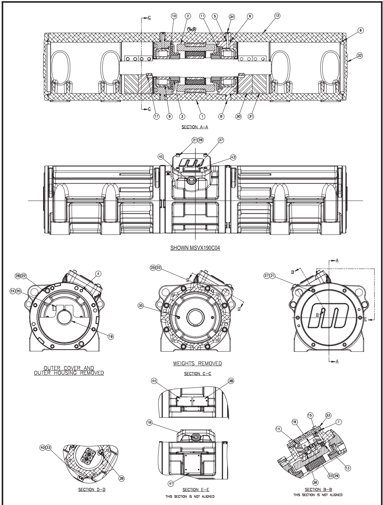
Figure 11. Martin® MSVX Screen Vibrator Part Numbers for MSVX190X04
