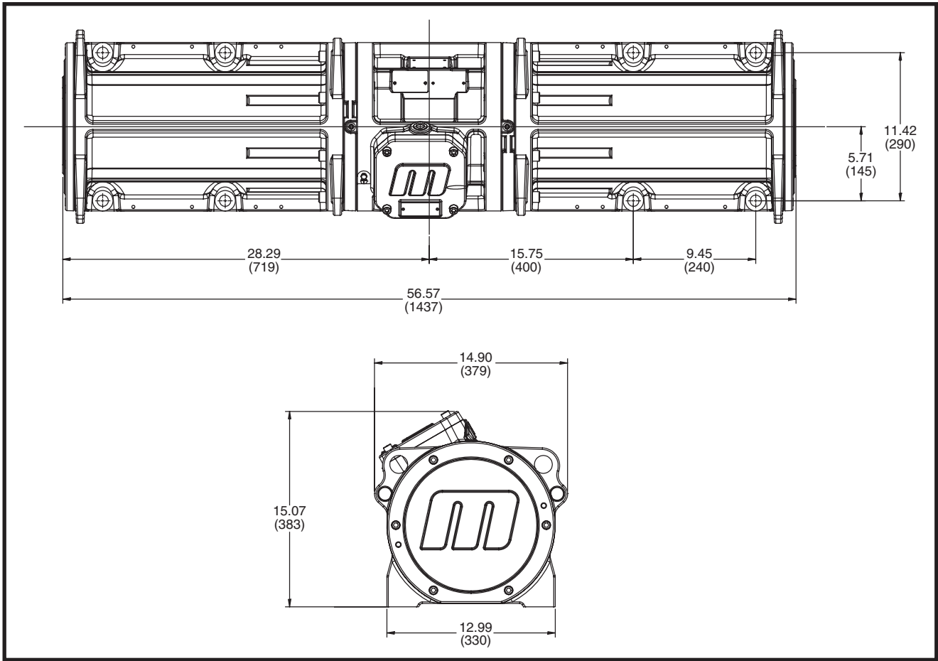
Figure 13. Martin® MSVX Screen Vibrator Dimensions, MSVX190X04
