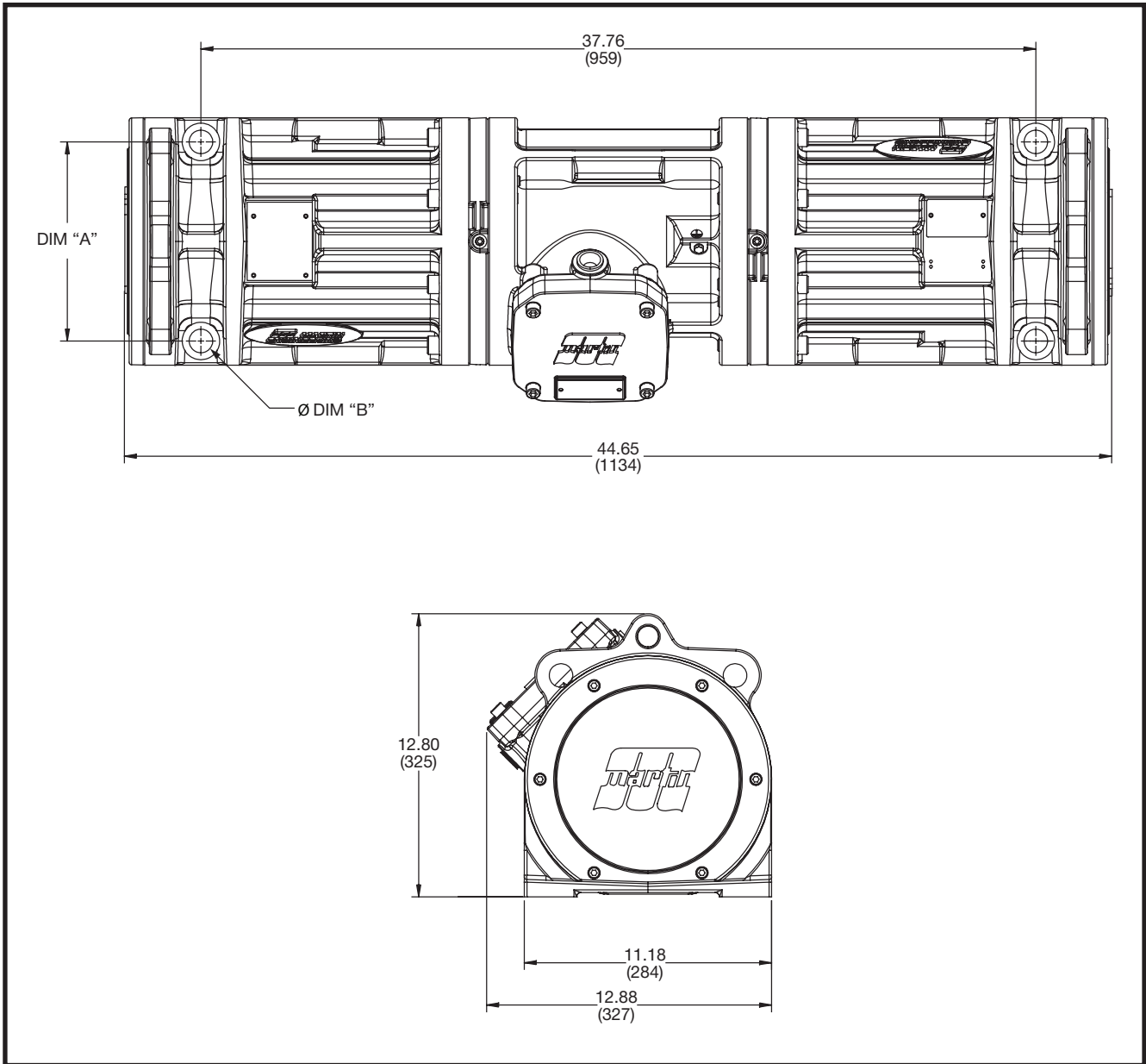
Figure 12. Martin® MSVX Screen Vibrator Dimensions, MSV70X02-XX, MSVX170X04-XX, and MSVX175X04-XX
