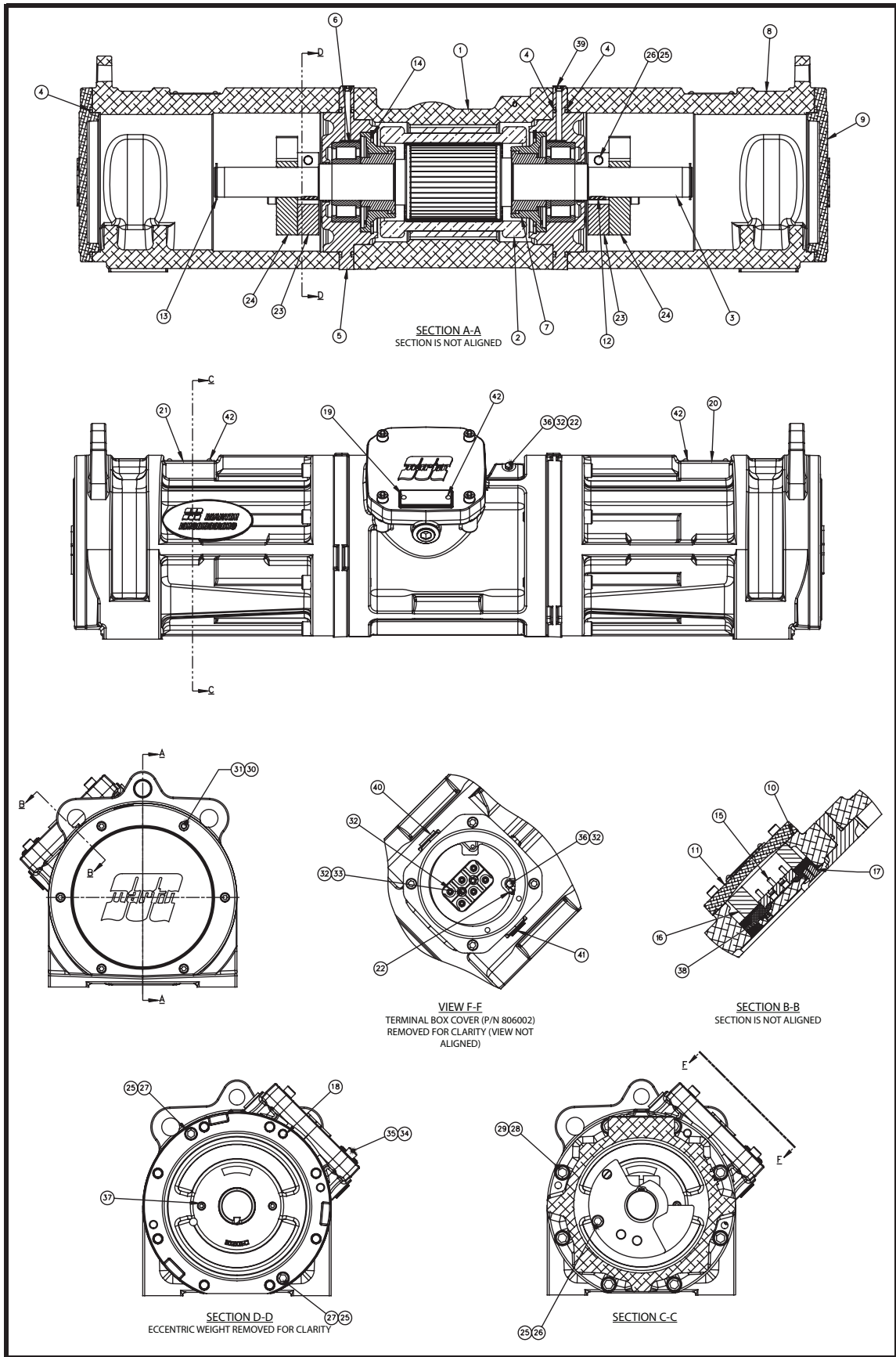
Figure 9. Martin® MSVX Screen Vibrator Part Numbers for MSV70X02-XX
