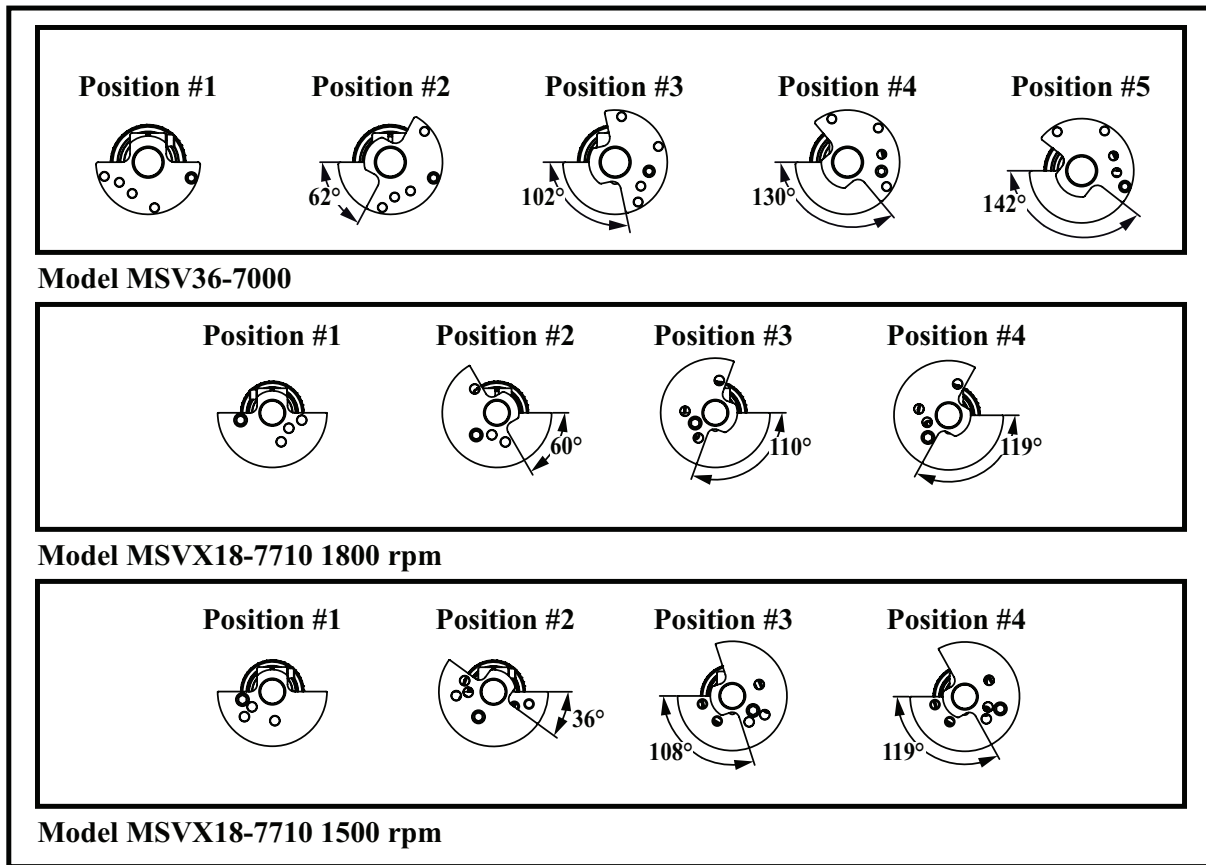
Figure 6. Vibrator Weight Settings
