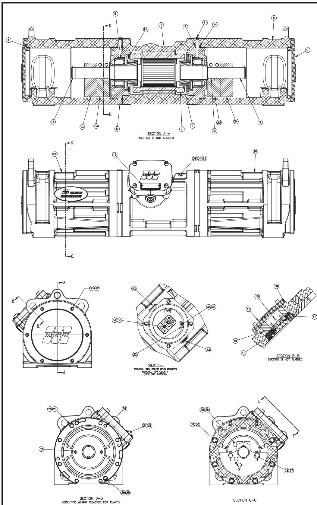
Figure 10. Martin® MSVX Screen Vibrator Part Numbers for MSVX170X04-XX & MSVX175X04-XX
