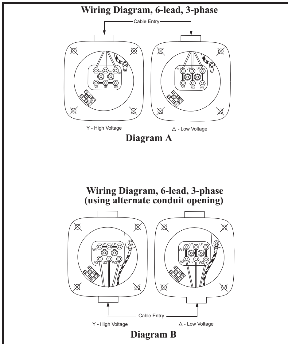
Figure 4. Wiring Diagrams
