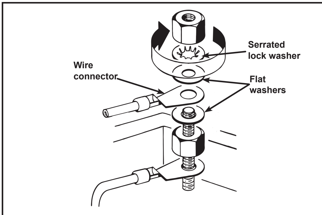
Figure 5. Installing Wire Connector
