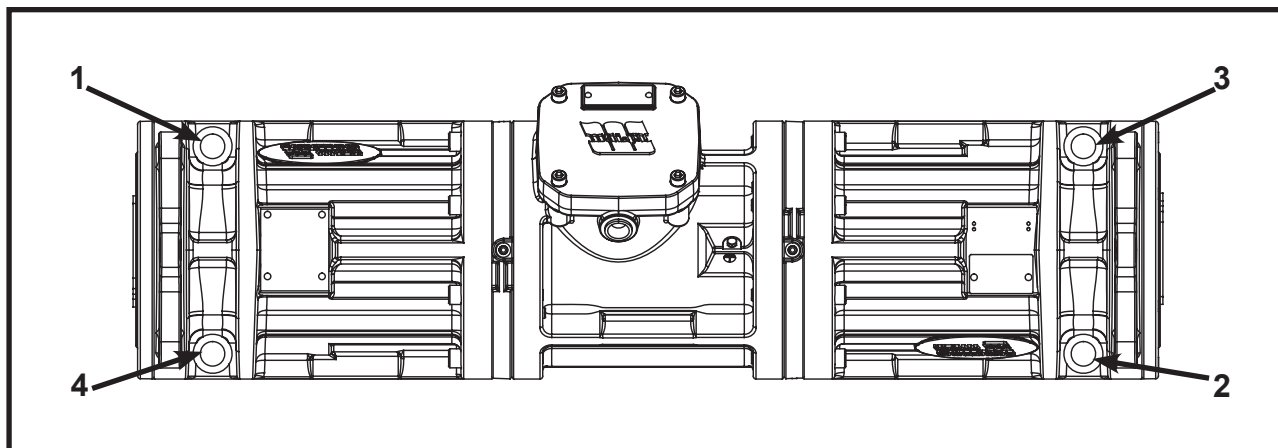
Figure 1. Mounting Bolt Tightening Sequence (4 Bolts)
