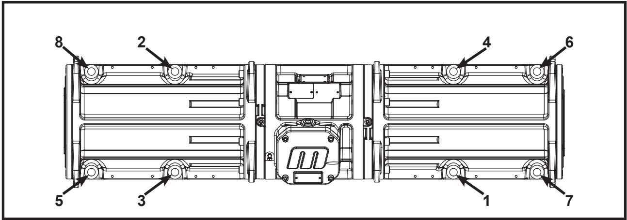
Figure 2. Mounting Bolt Tightening Sequence (8 Bolts)
