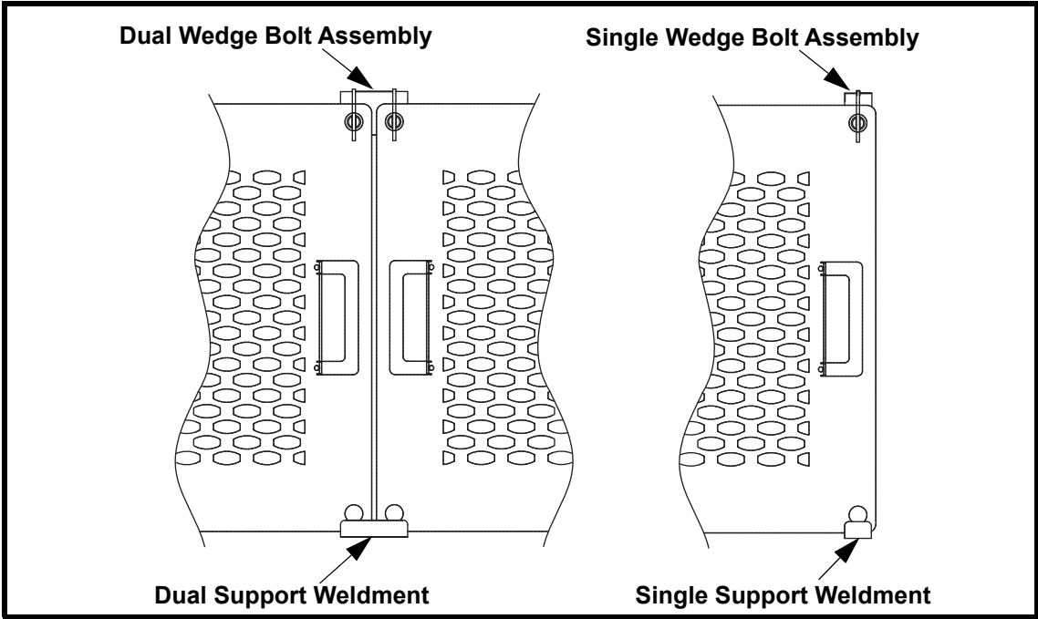
Figure 2. Installation Configurations
