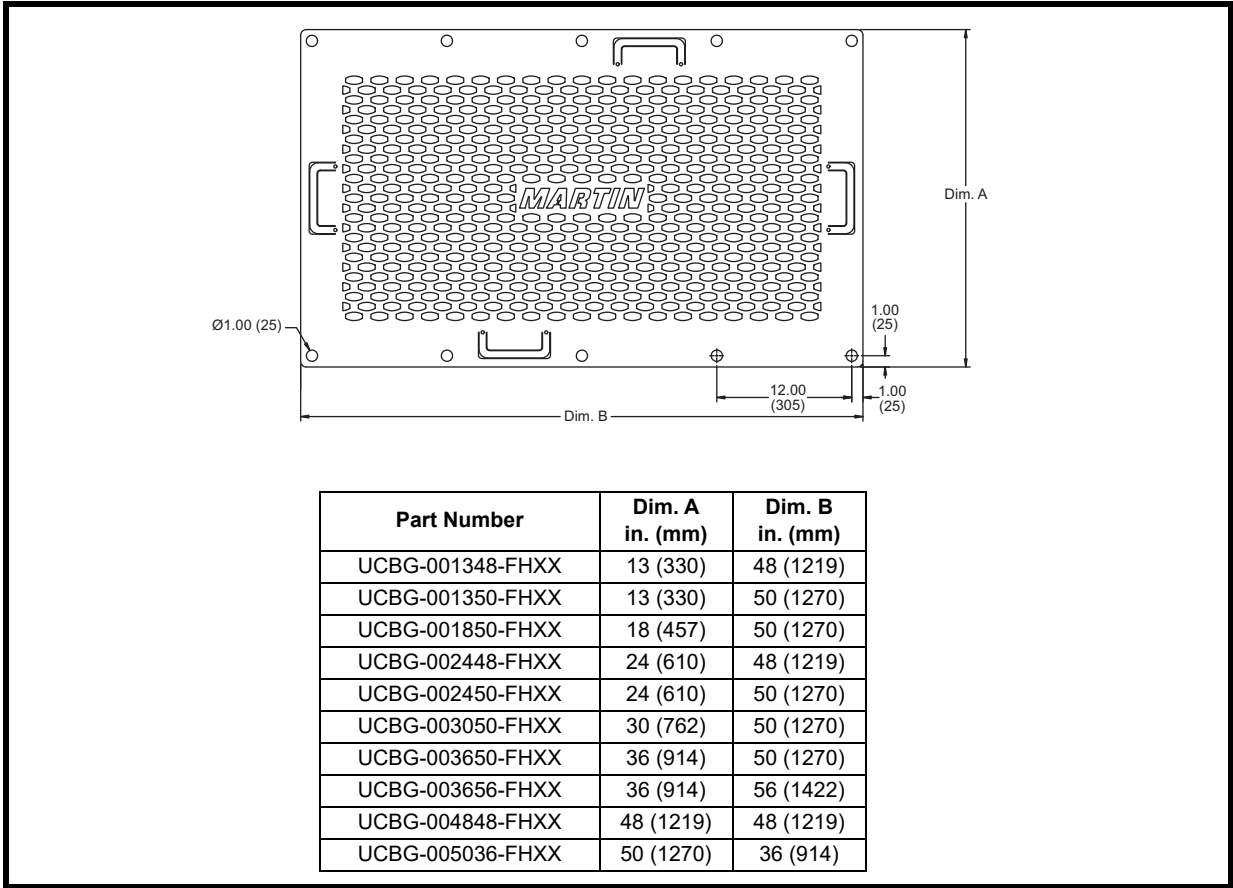
Figure 1. Conveyor Guard Dimensions
