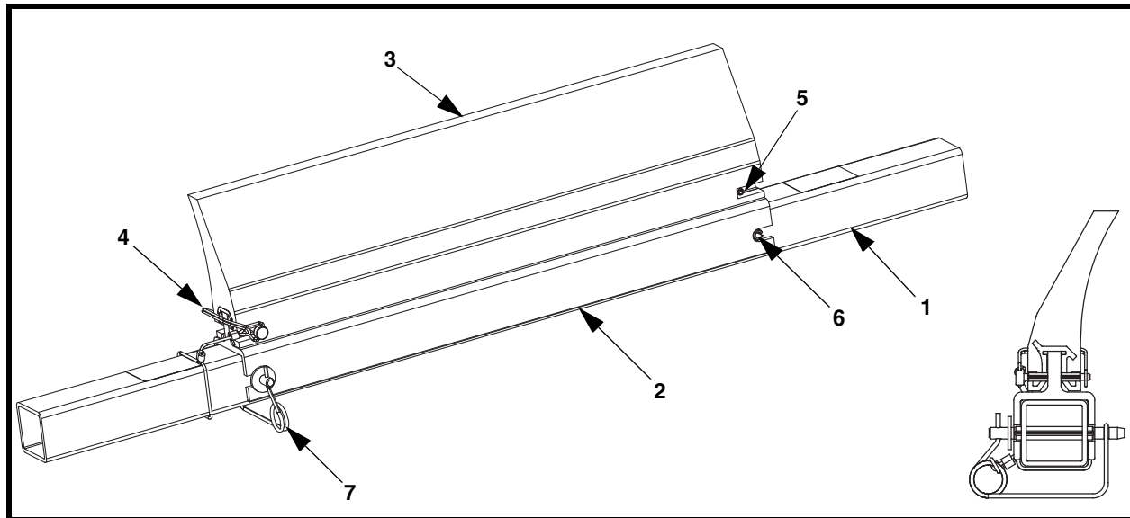
Martin® H2O Cleaner Assembly, P/N H2O4000S-XXXX
